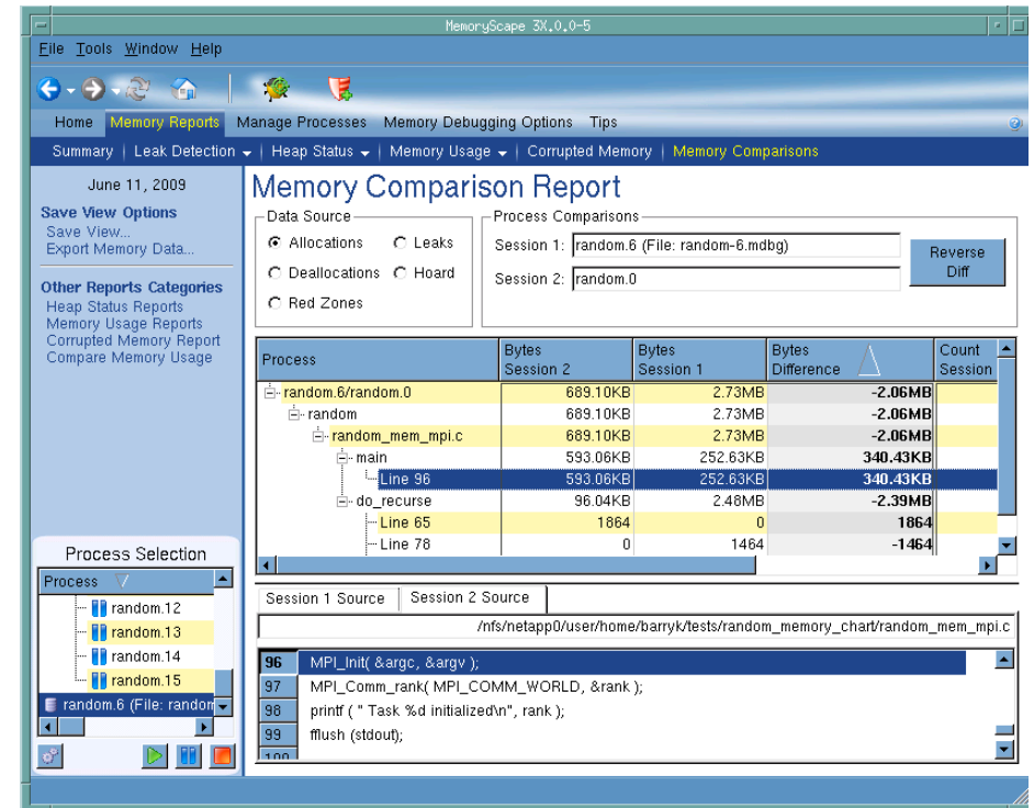
Figure 19: Memory Comparison Report
