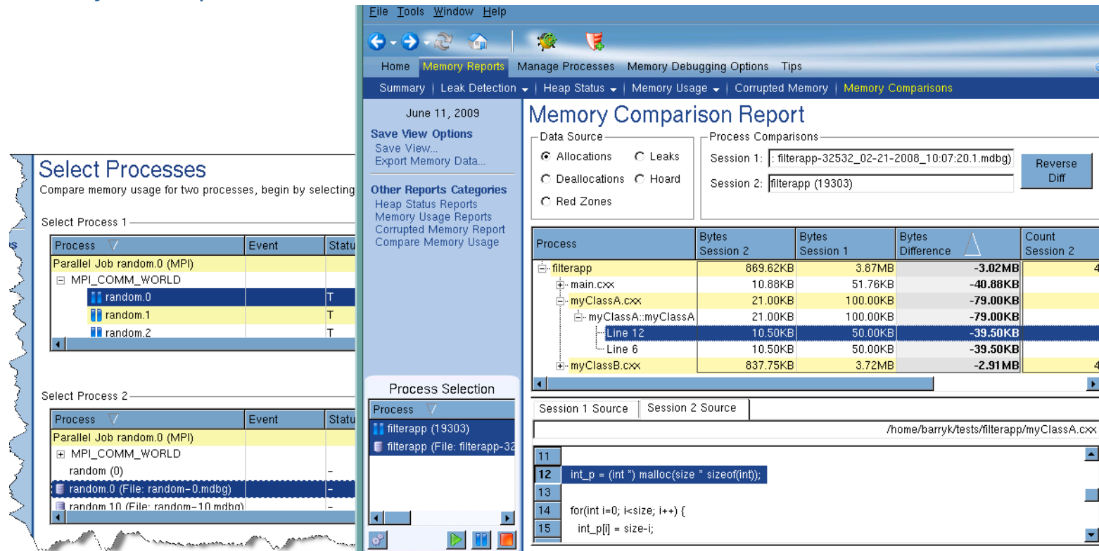
Figure 71: Memory Use Comparisons
