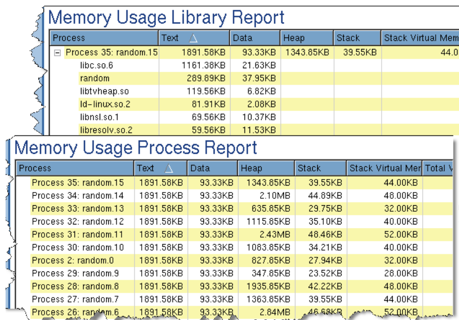
Figure 53: Memory Usage Library and Process Reports
