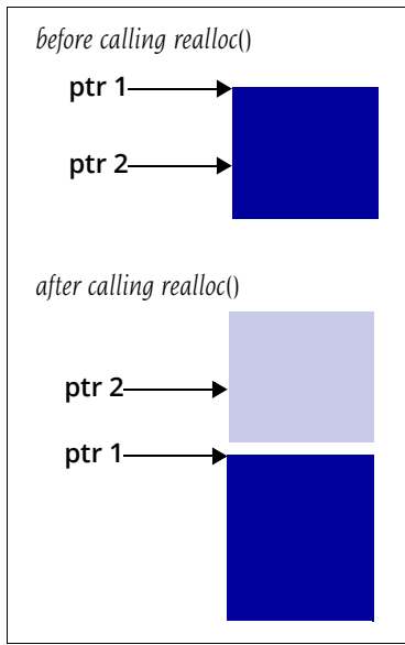
Figure 13: realloc() Problem
