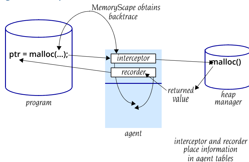
Figure 5: Interposition
