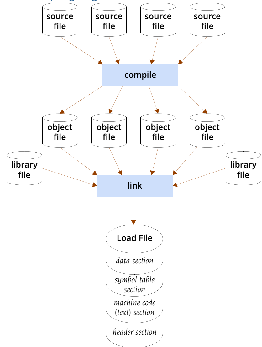
Figure 2: Compiling Programs
