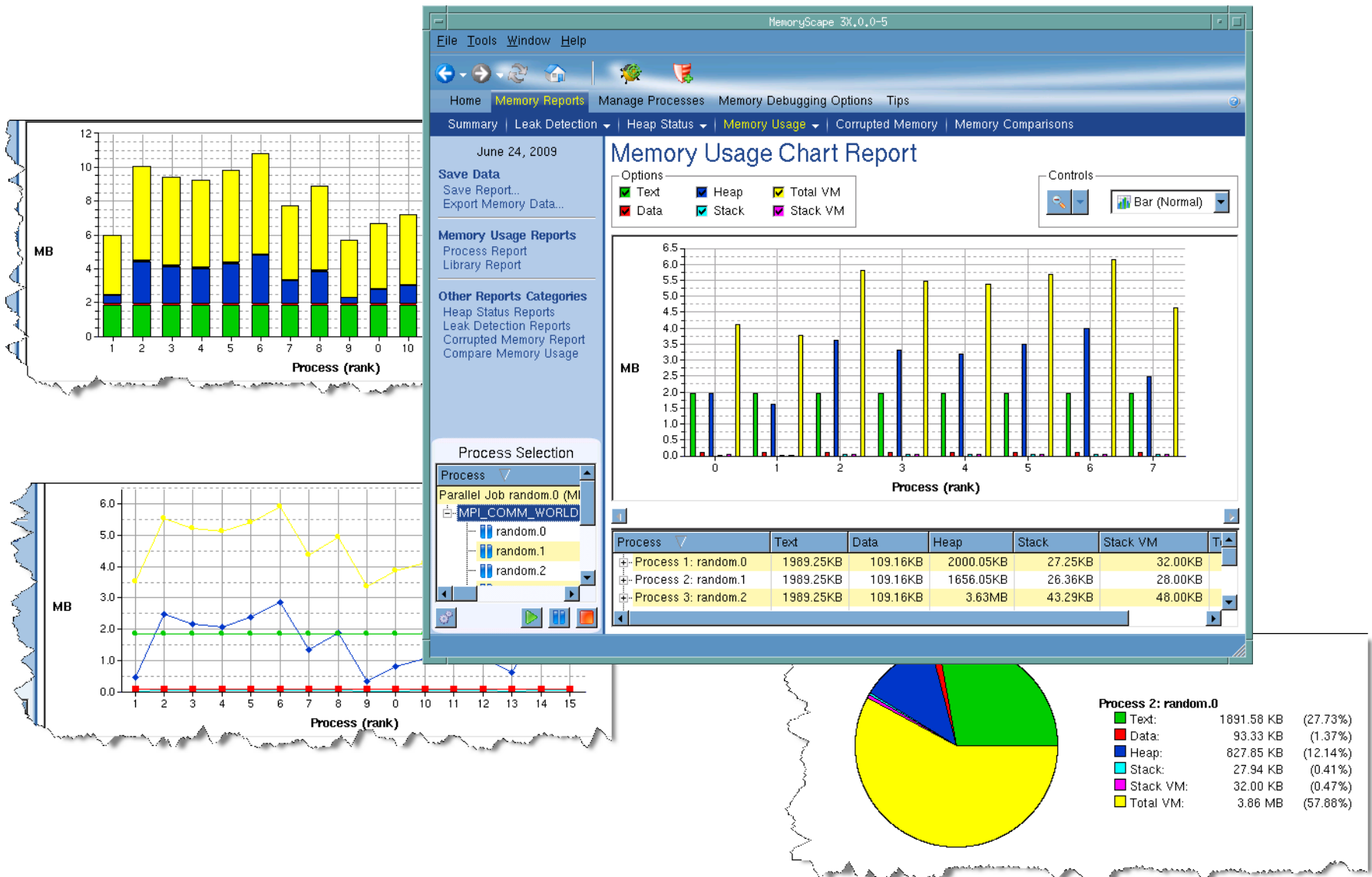
Figure 54: Memory Usage
