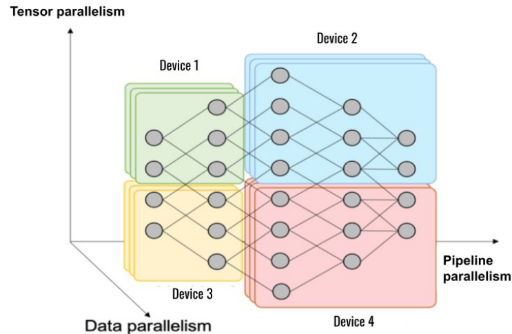
Model Parallelism
