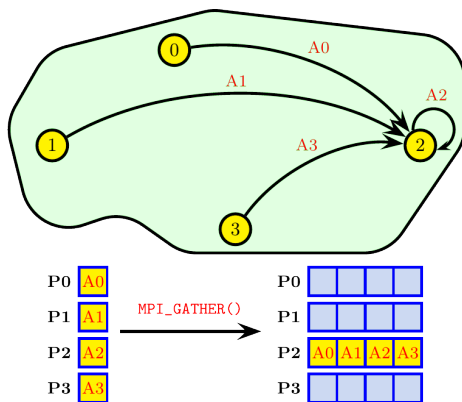
Figure 15 – Collection : MPI_Gather()
