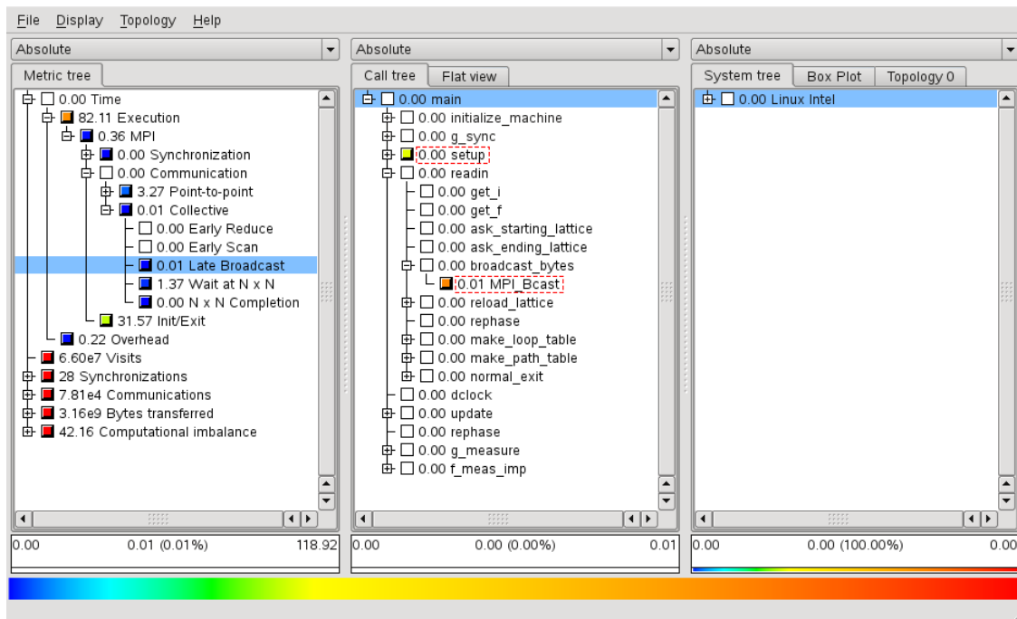
Figure 4.1.: Dashed red frames guide the user in locating the call paths where the most severe instances of the wait states detected by Scalasca (here: Late Broadcast) occurred.
