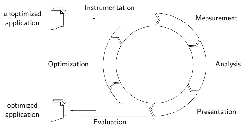
Figure 1.1.: Performance optimization cycle
