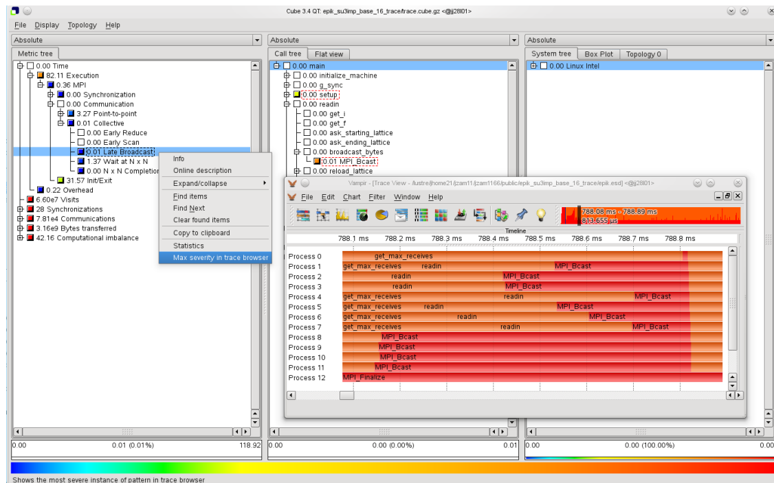
Figure 4.2.: Location of the worst Late Broadcast instance shown in the timeline display of Vampir. It can be seen that some processes enter the MPI_Bcast operation earlier than the root process. It is leading to a wait state.
